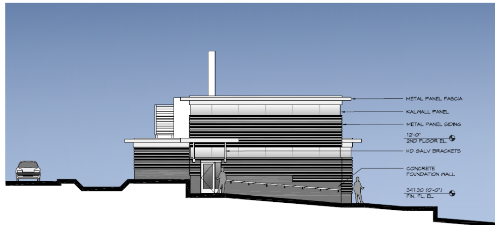
EAST ELEVATION
