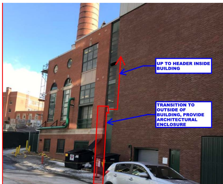
Steam Entry point at the CUP
