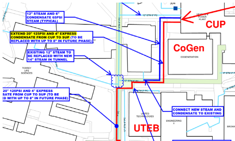
Steam Path from Gant back to the CUP
